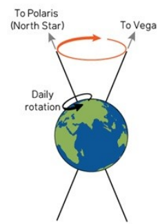
Orbital Precession 26,000 yrs
